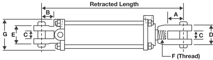
Dimensional Data for Lion TH Cylinders
