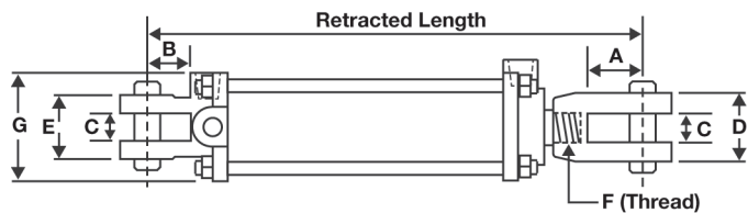
Dimensional Data for Lion TH Cylinders
