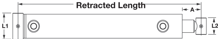
Dimensional Data for Prince Cylinders on this page
