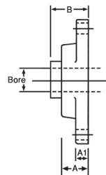
Side UCFL
