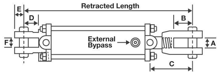
Dimensional Data for Prince Rephasing Cylinders
