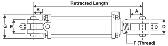
Dimensional Data for Lion TH Cylinders
