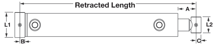
Dimensional Data for Prince "Royal" Cylinders
