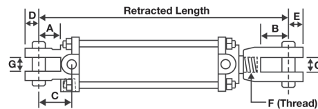
Dimensional Data for Prince Tie Rod Cylinders
