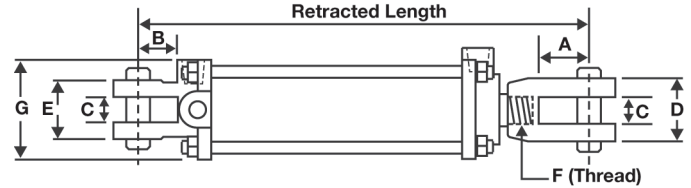
Dimensional Data for Wolverine Cylinders
