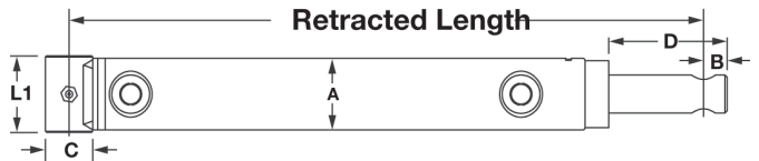
Dimensional Data for Surplus Center Welded Cylinders
