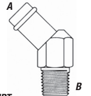
Hosebarb M to NPT M 45° Elbow 300 PSI max.
