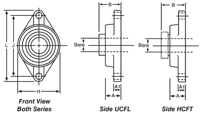
Side UCFL
