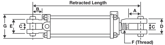
Dimensional Data for Maxim Cylinders
