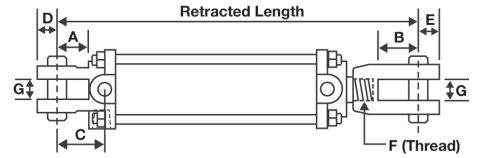
Dimensional Data for Prince Tie Rod Cylinders
