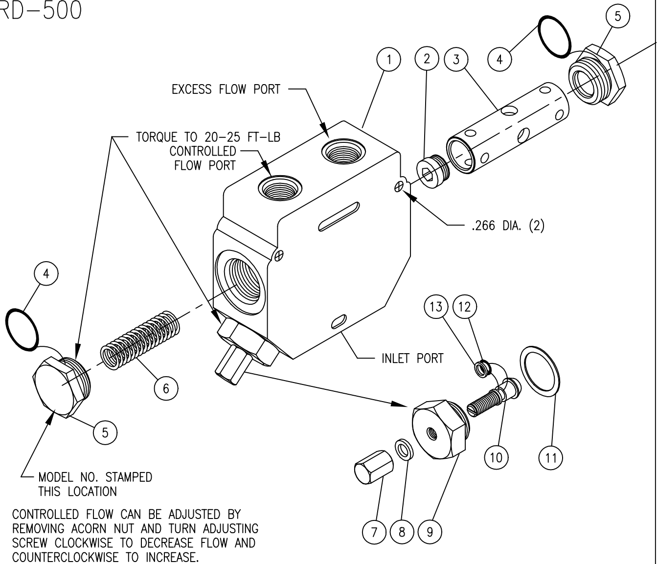
RD-500 ADJUSTABLE FLOW PRIORITY DIVIDER
