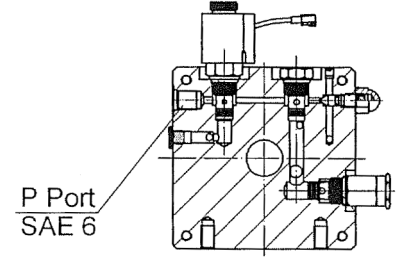
Section M-M
