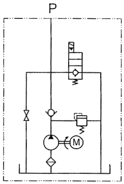
HYDRAULIC SCHEMATIC
