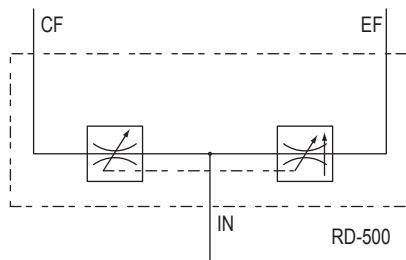
Circuit Symbol
