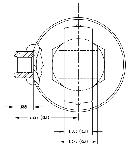
ROD END VIEW
