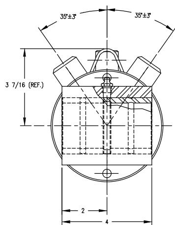
ROD END VIEW
