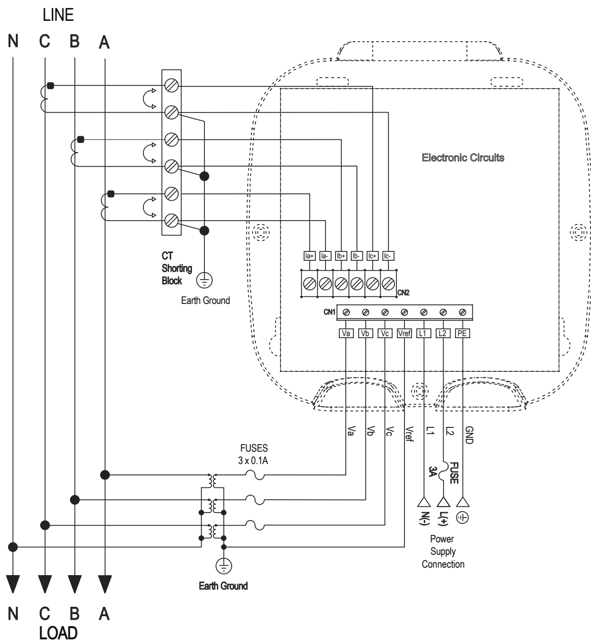
3 PHASE 4 WIRE WYE WITH PTS
