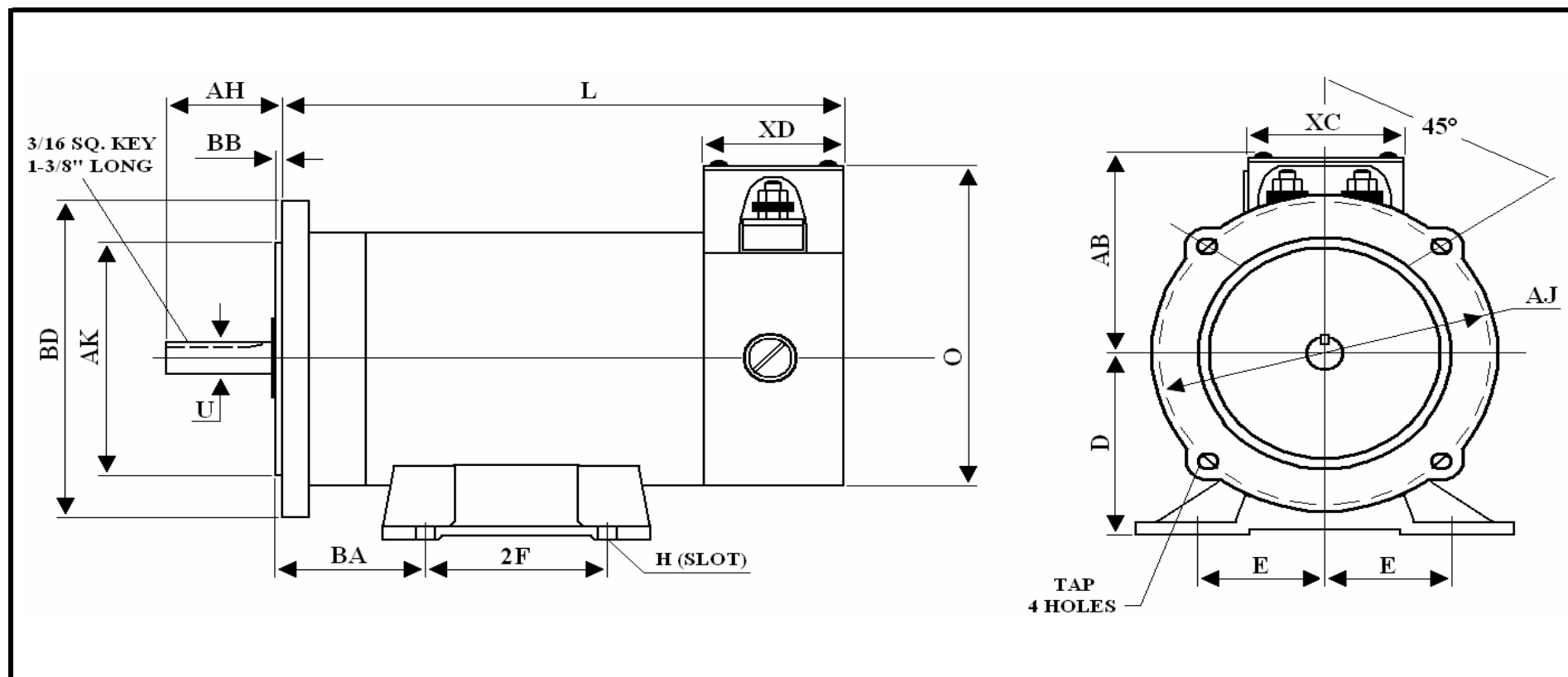
DIMENSIONS - Inches
