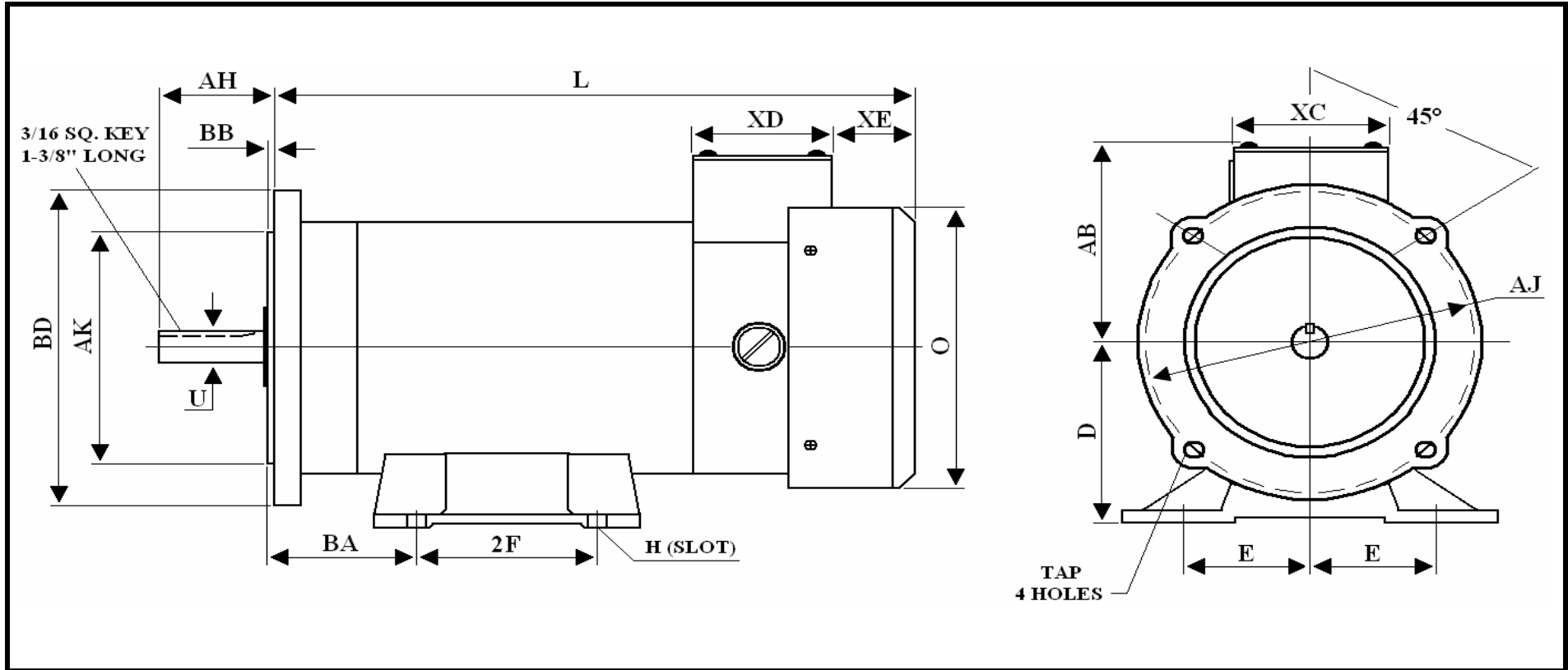
DIMENSIONS - Inches
