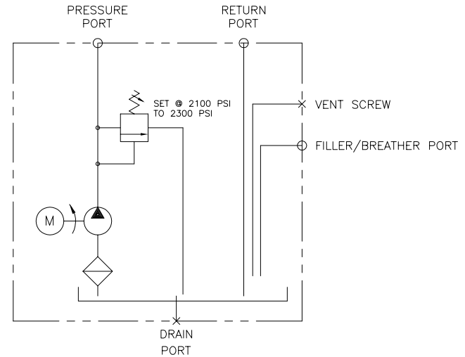
HYDRAULIC SCHEMATIC
