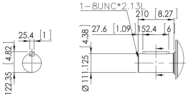
Output Shaft
