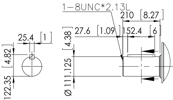
Output Shaft
