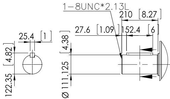
Output Shaft
