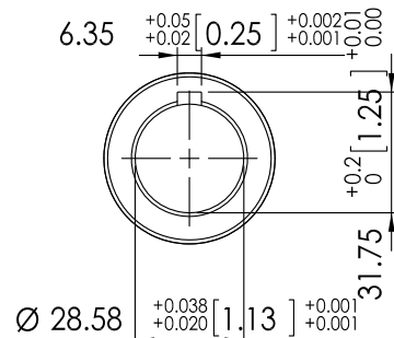
input bore
