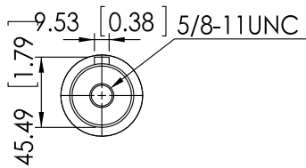
output shaft
