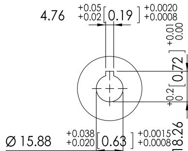
input bore
