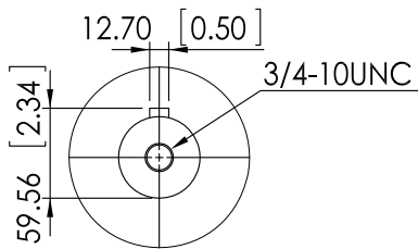
output shaft
