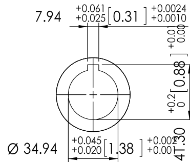
input bore
