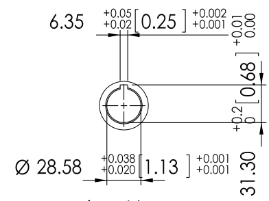
input bore
