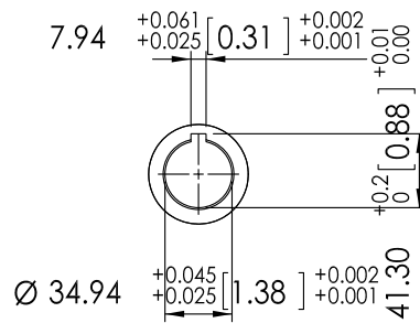
input bore
