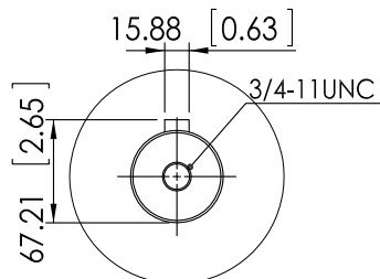
output shaft
