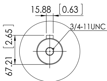
output shaft
