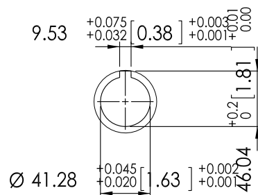
input bore
